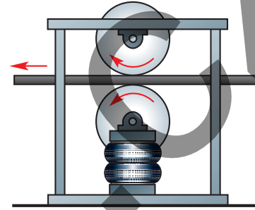
Roller tensioning
