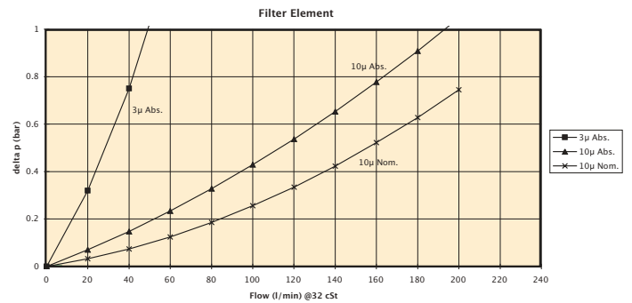
Filter Element
