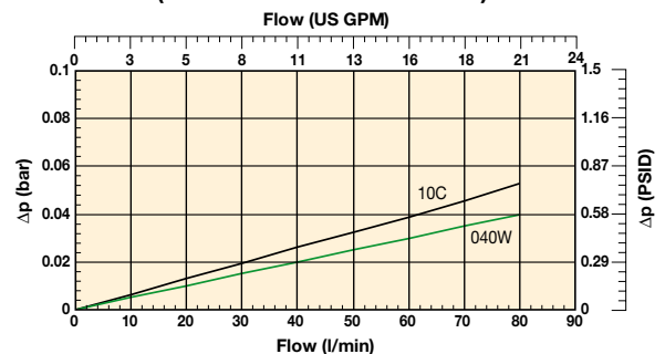
TPR80 (Element length code 2) (cellulose and stainless steel)
