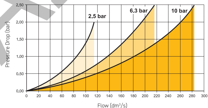
(3/4") Adsorber Filter
