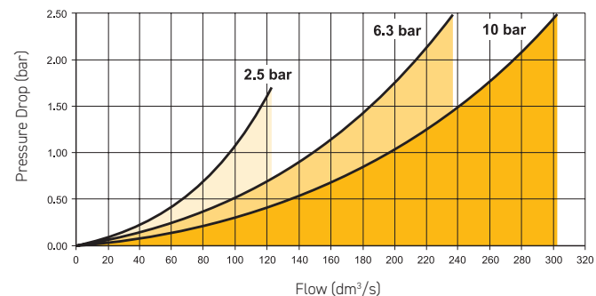
(1") Adsorber Filter
