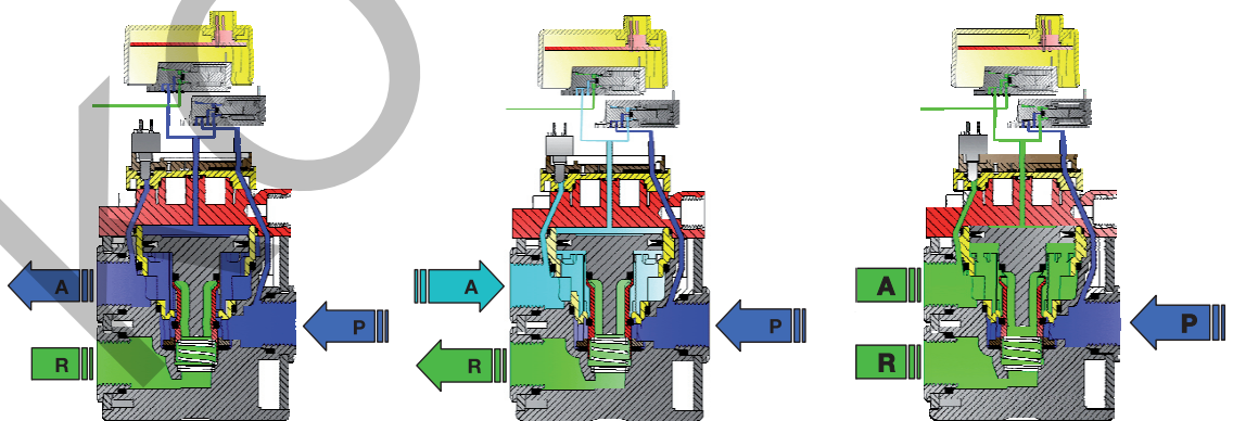
Filling position
