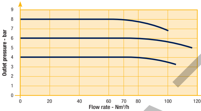
Flow Curve 1/4"
