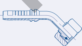
45° Swept Female Metric Light Serie 24° Cone Seat Swivel (DKOL 45)
