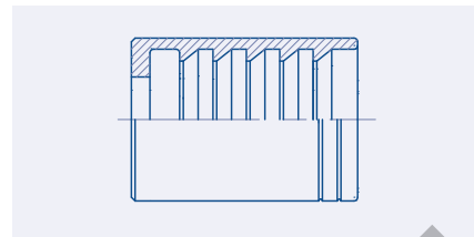
NON SKIVE Balfit® 2 Wire Braid Ferrule
